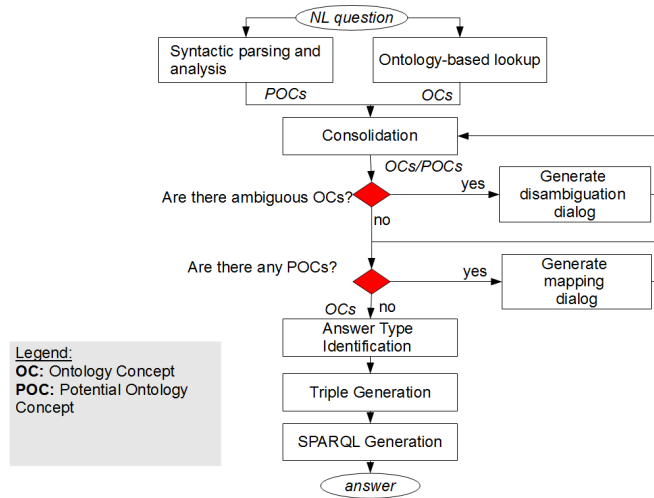
Fig. 1. FREyA Workflow
