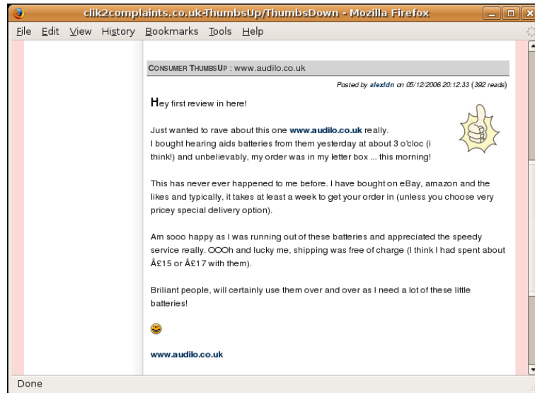
FIG. 3 – Positive/Negative reviews
