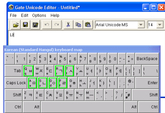
Figure 4: The GUK Unicode editor using a Korean virtual keyboard.
