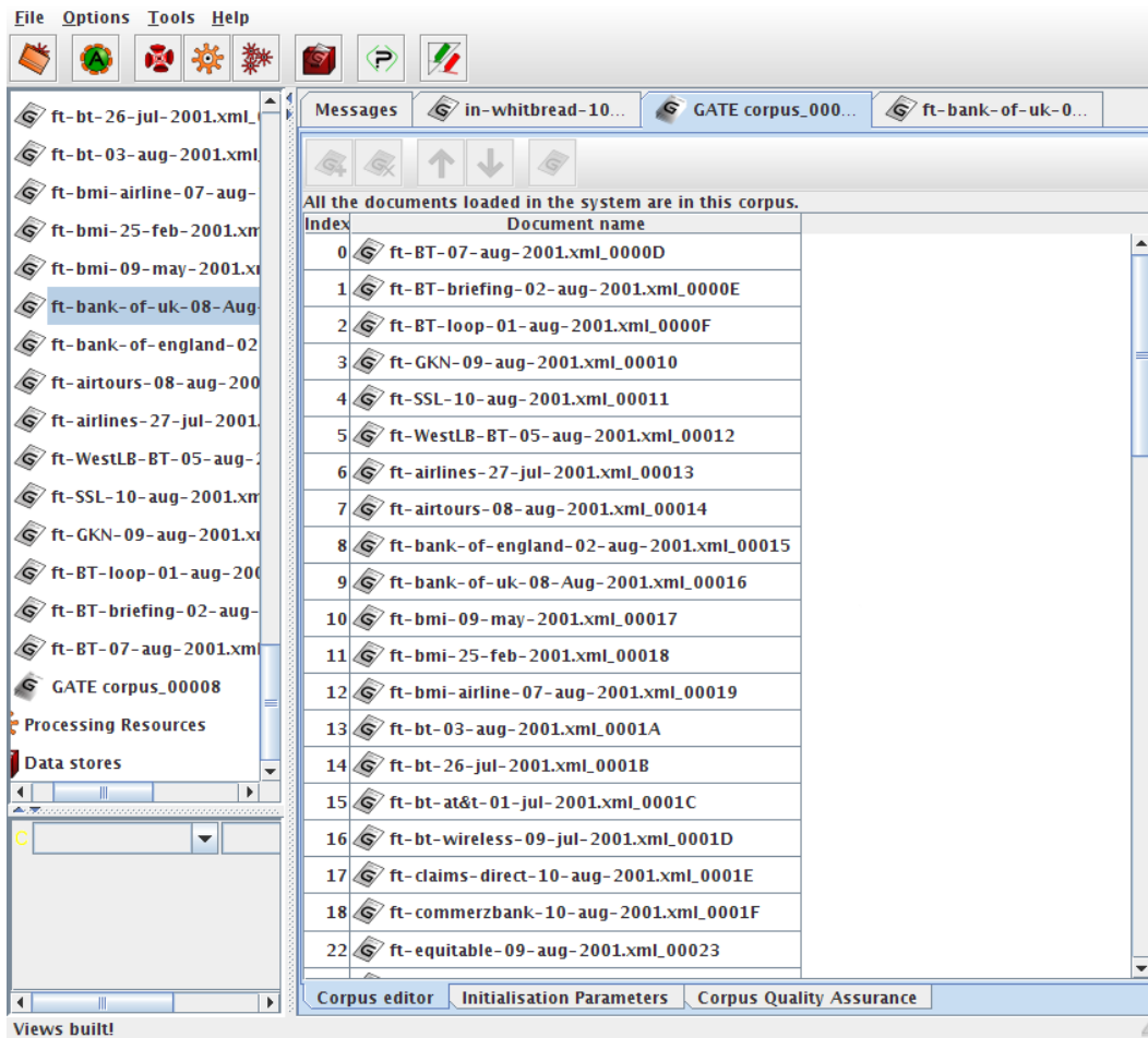
Figure 3.5: Corpus Editor
