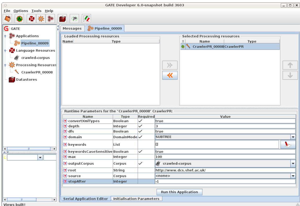
Figure 23.5: Crawler parameters
