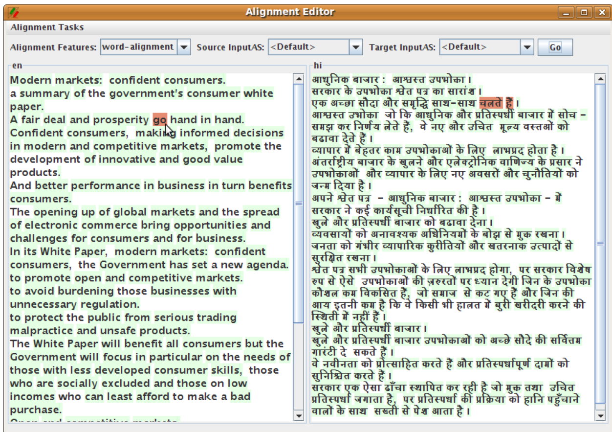
Figure 20.3: Alignment Viewer
