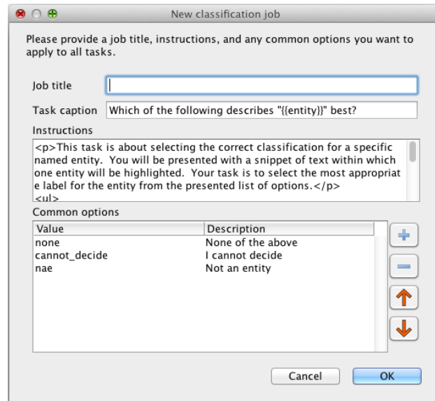
Figure 21.1: Setting options to create a new classification job
