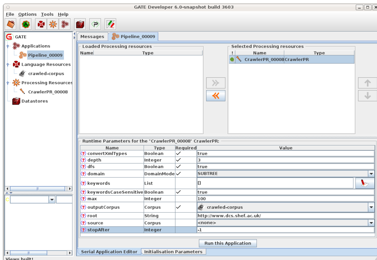
Figure 19.3: Crawler parameters
