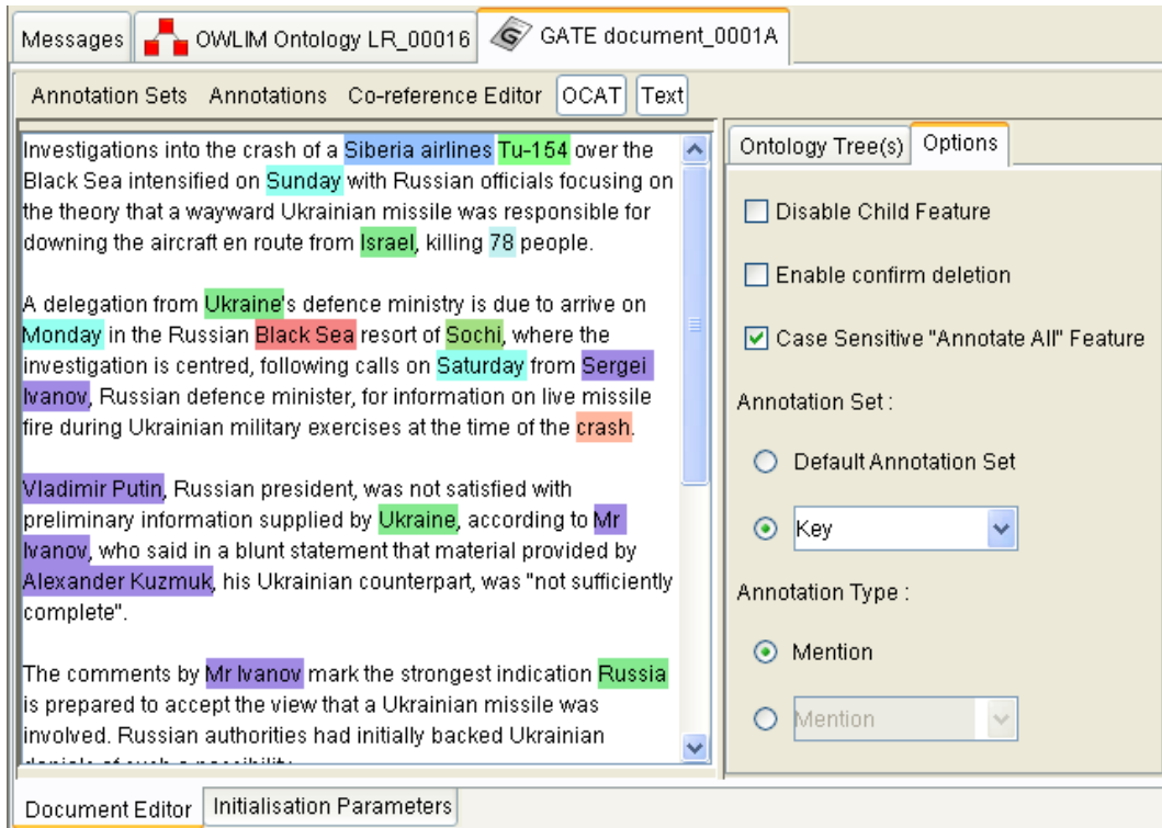
Figure 14.11: Tool Options
