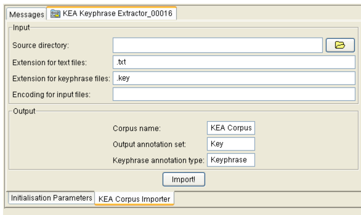
Figure 19.8: Options for the ‘KEA Corpus Importer’
