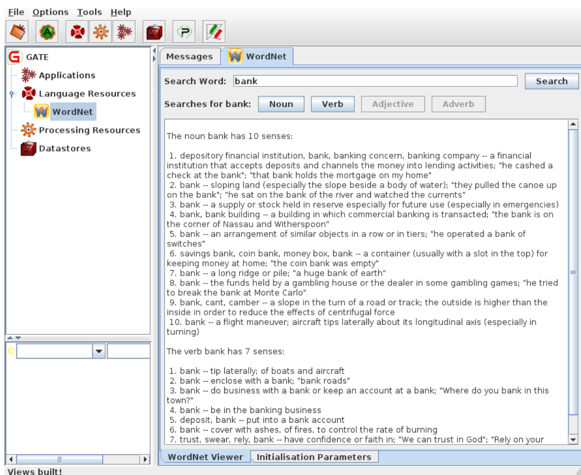
Figure 19.4: WordNet in GATE – results for ‘bank’
