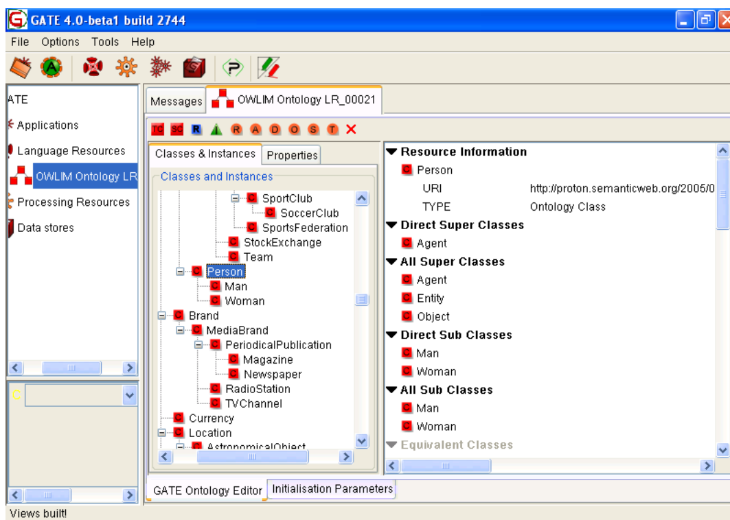
Figure 14.7: The GATE Ontology Viewer
