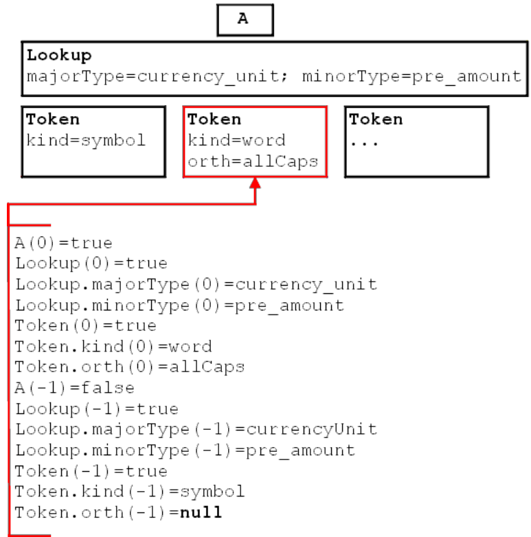
Figure 15.1: Sample attributes and their values
