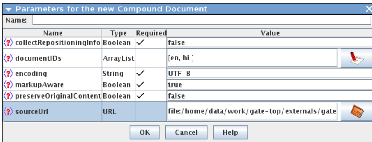
Figure 16.1: Compound Document
