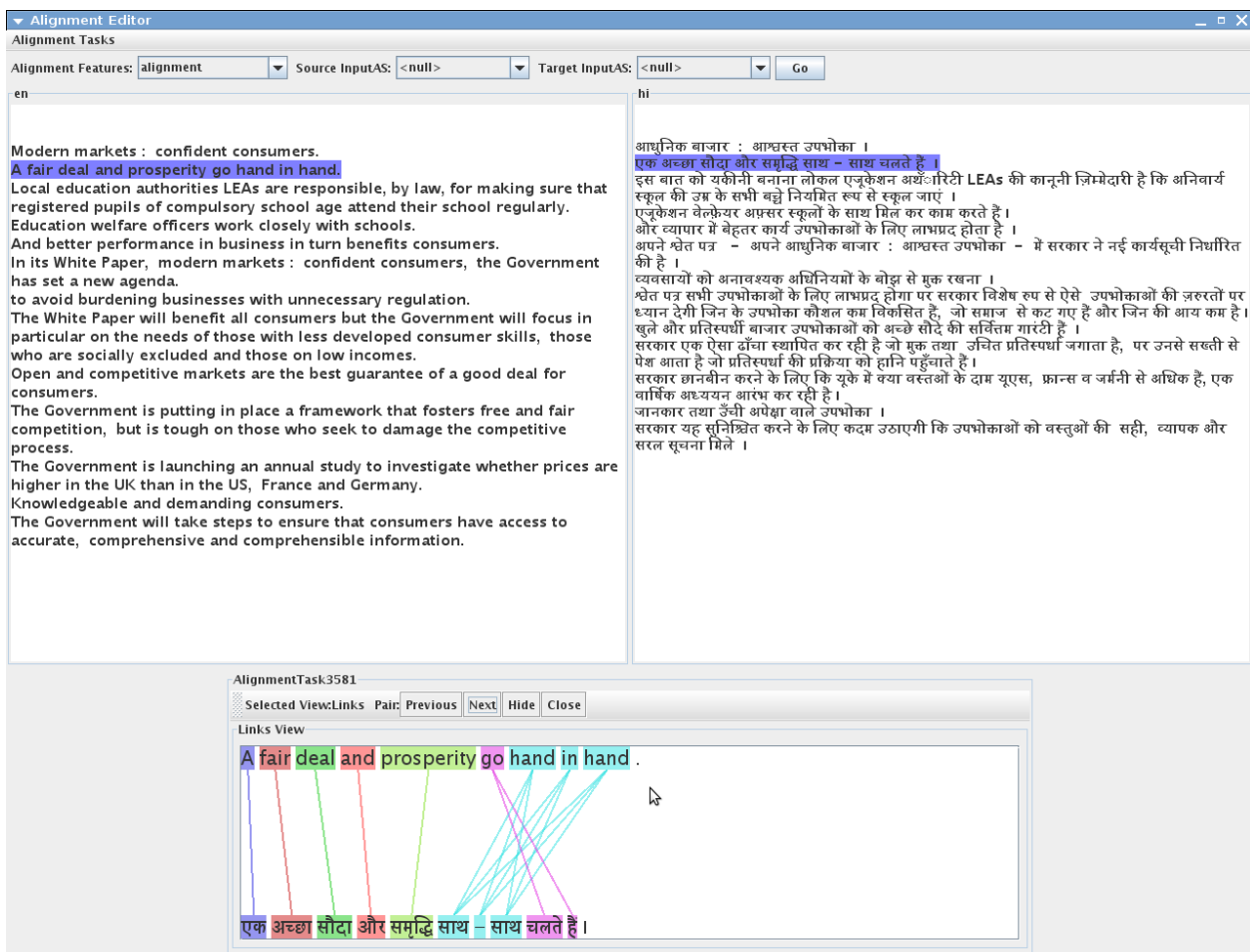
Figure 16.4: Links View
