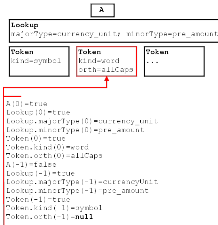
Figure 8.8: Sample attributes and their values
