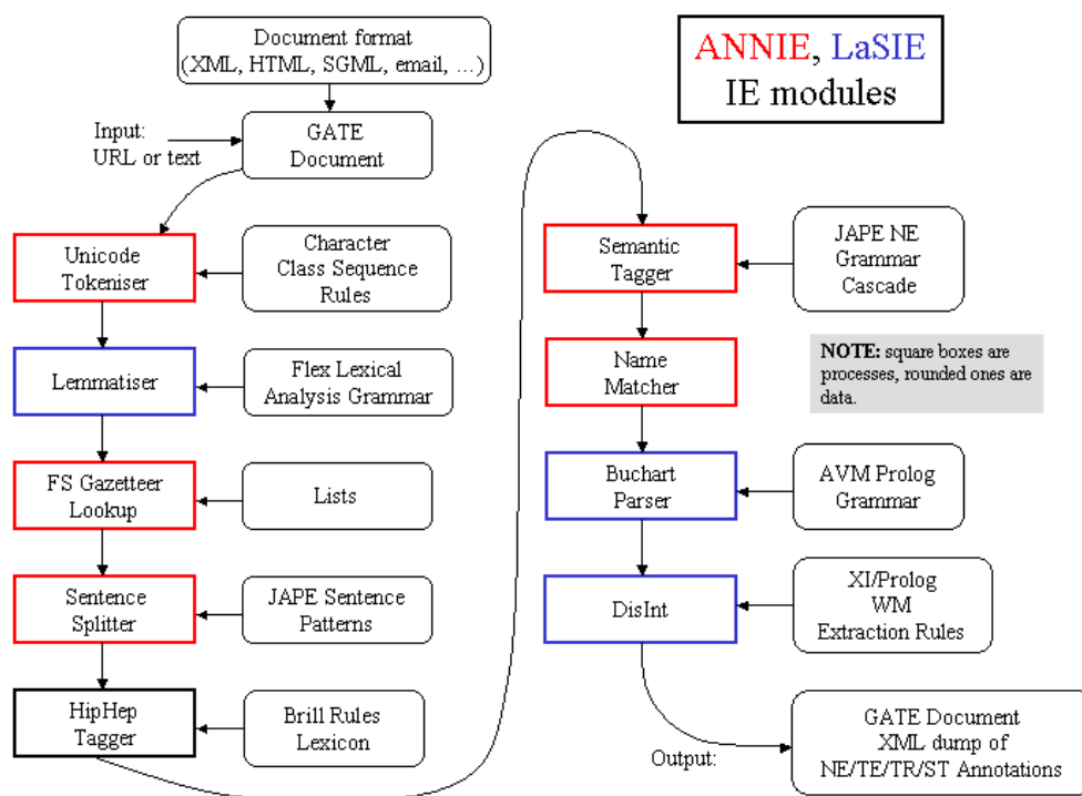
Figure 7.1: ANNIE and LaSIE
