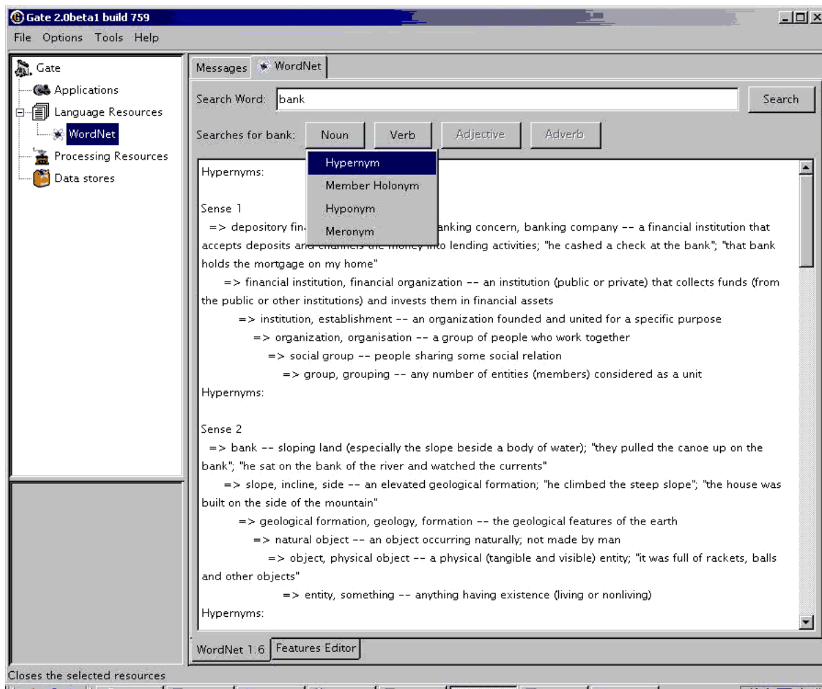
Figure 8.6: WordNet in GATE
