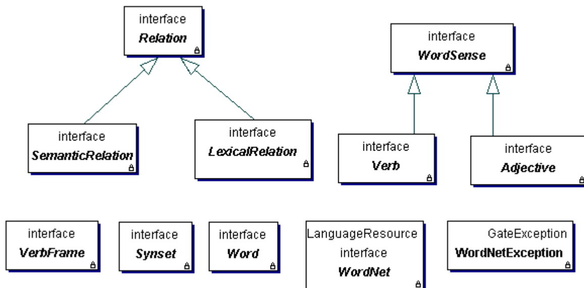
Figure 8.7: The Wordnet API
