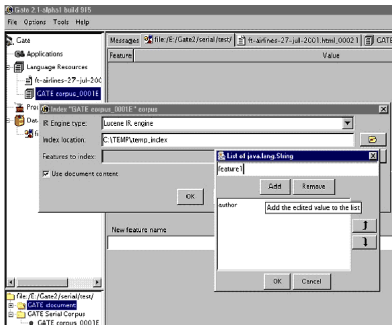
Figure 8.4: Indexing a corpus by specifying the index location and indexed features (and content)
