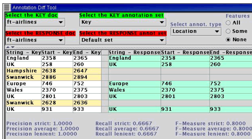
Figure 9.1: Part of the AnnotationDiff viewer
