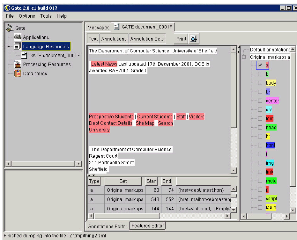
Figure 2.1: Main Window
