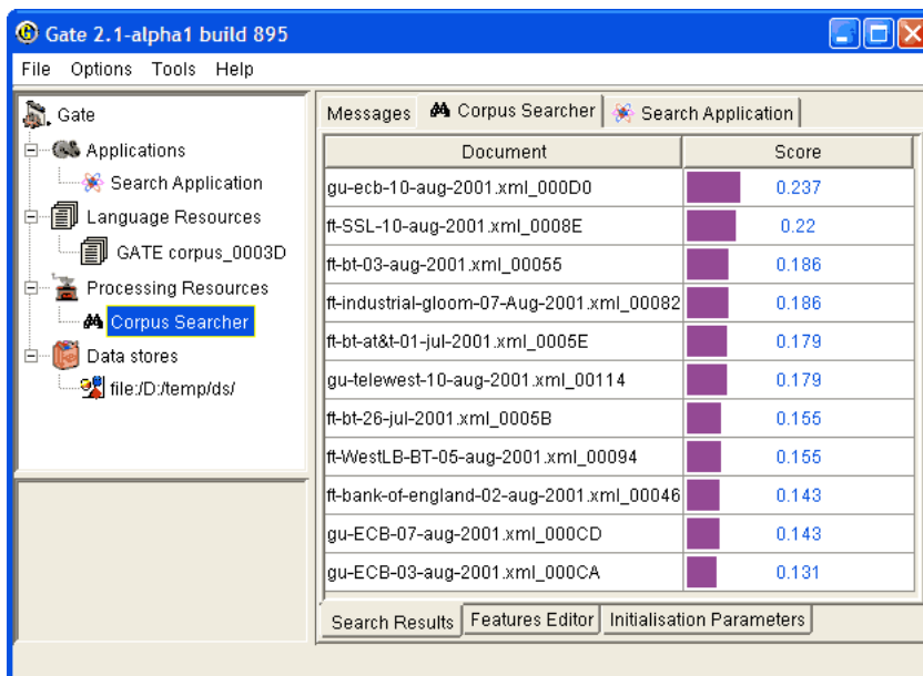
Figure 8.3: Documents with scores, returned from a search over a corpus
