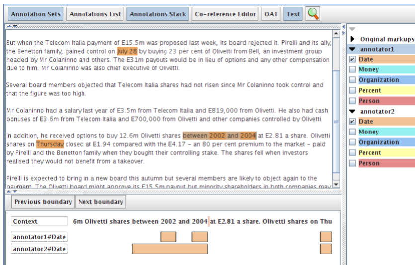
Fig. 3 Part of the adjudication user interface, showing the document displayed with highlighted annotations and annotation stack and list displays to the bottom and right, allowing different annotators' work to be compared by the adjudicator
